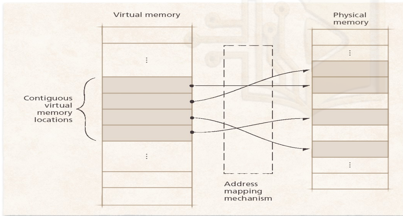
Figure 5.5 Artificial contiguity.
